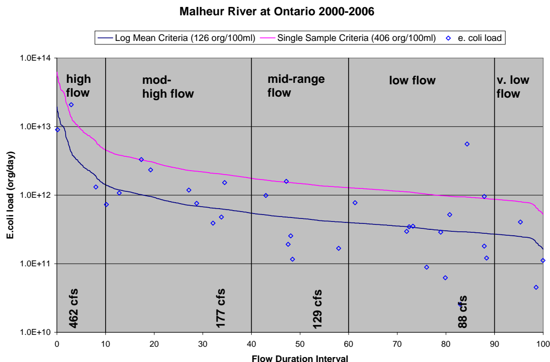
Figure A-2. Load duration curves with measured daily loads and selected flow ranges, Malheur River in Ontario. Points located above curves exceed standards. Sample location is Hwy 201 bridge near mouth of river and flow gauge is at 36th Street Bridge, approximately two miles upstream.
