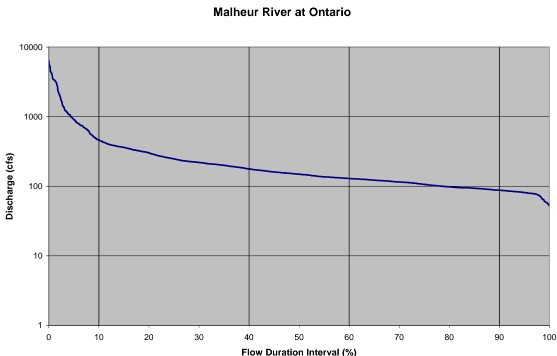
Figure A-1. Flow Duration Curve, Malheur River at Ontario.
