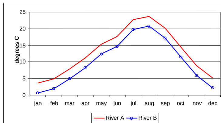
Figure 7-1: Two Temperature Profiles
