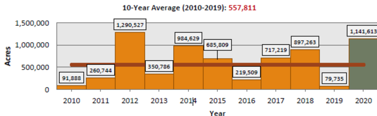
Figure 1. Wildfire acres burned in Oregon, 2010-2020.
