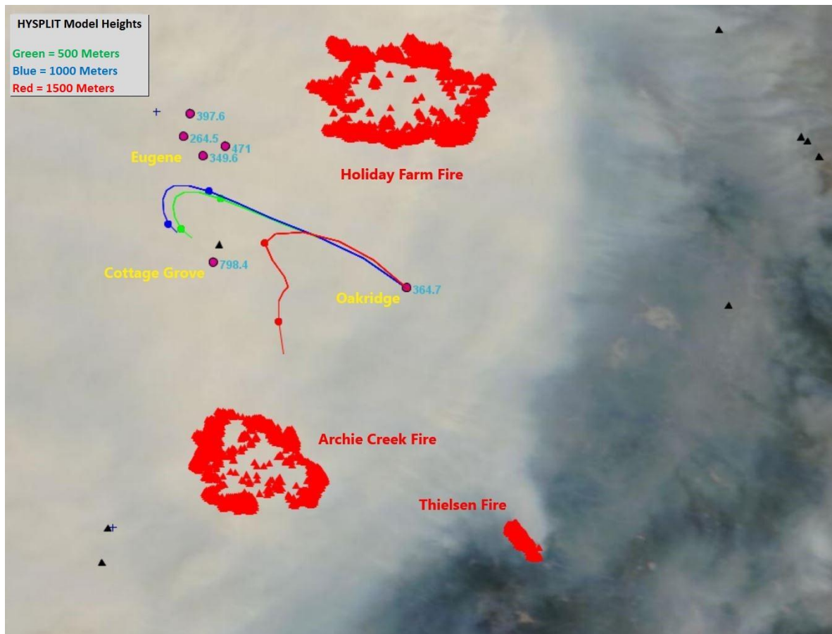
Figure 12. Satellite Smoke and back trajectory HYSPLIT Model Image, 9/10/2020
