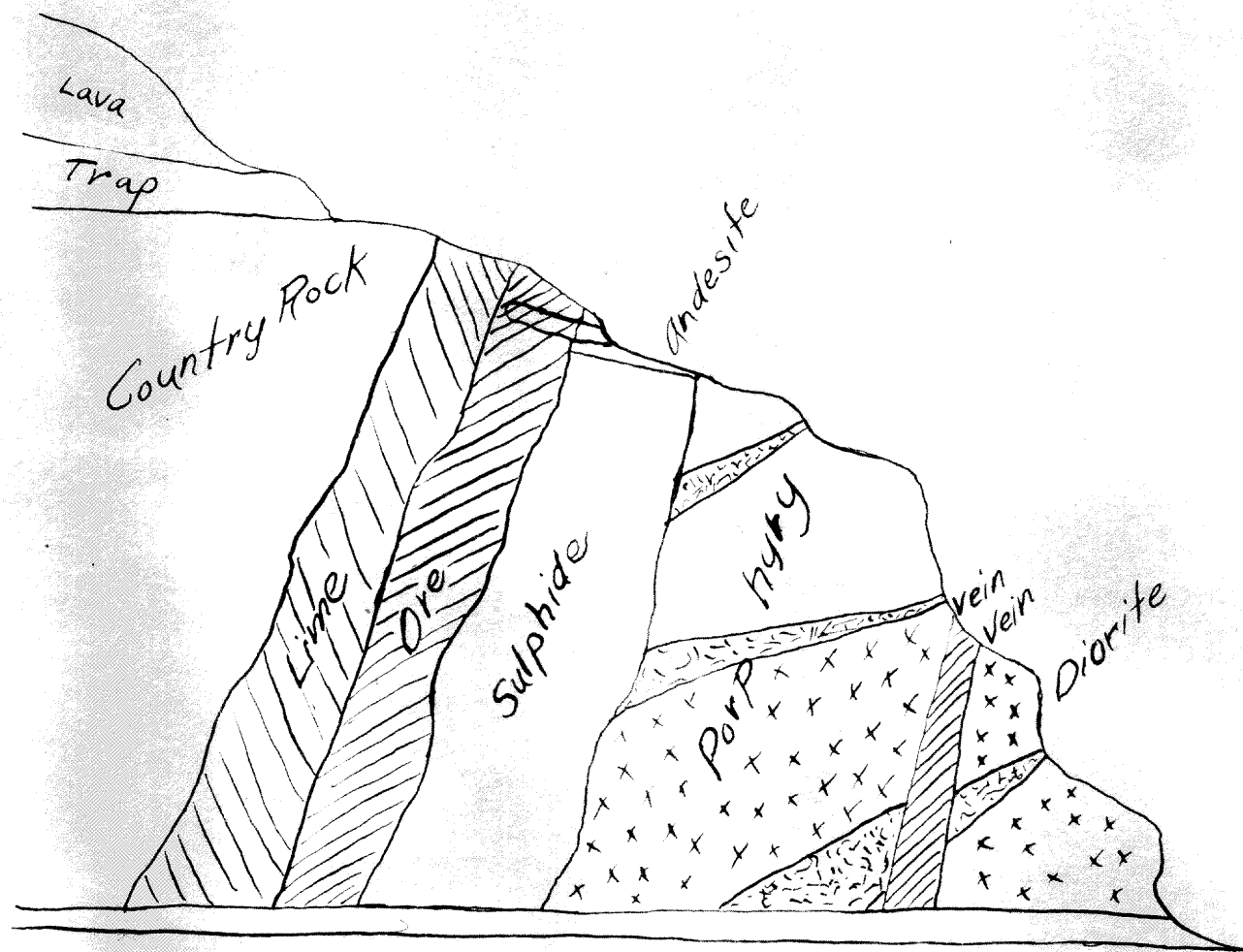
~ Gross section of Squaw Creek Mineral Belt
